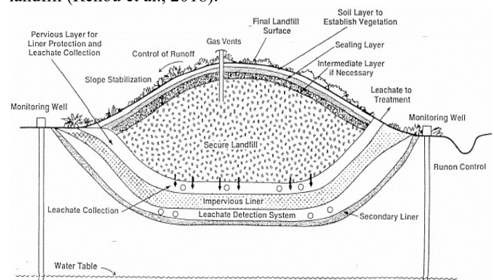
Fig. 1 A schematic view of a landfill (Qrenawi et al., 2011)
